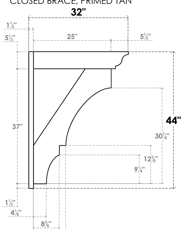
SIDE PROFILE
